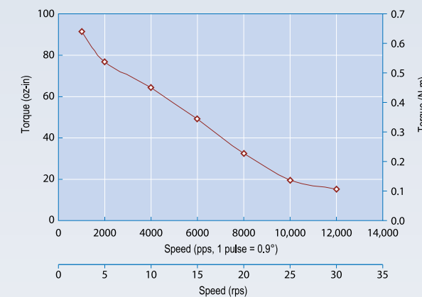
CO-5718M-02P 24VDC, 3.0 Amps Peak, SilverPak 23C, 1/2 Stepping
