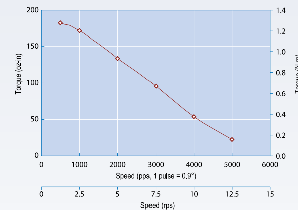
CO-5718L-01P 24VDC, 3.0 Amps Peak, SilverPak 23C, 1/2 Stepping
